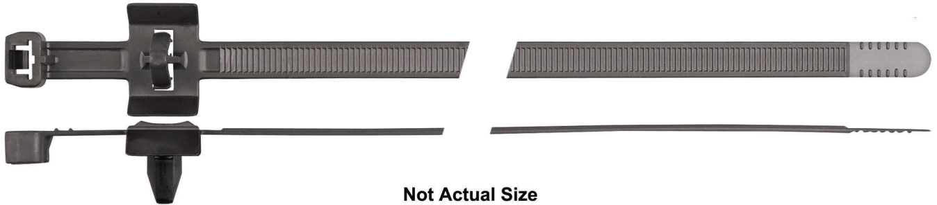
15151PK 5/16" (8mm) Hole Size 25 Pcs. 200mm Overall Length 55mm Max Bundle Diameter Black Nylon Releasable Cable Straps Nissan # 24225-89960
