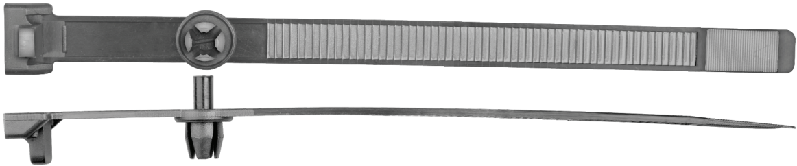
15714PK 5/16" (8mm) Hole Size 10 Pcs. 6 3/8" (160mm) Length Black Nylon Releasable Cable Ties Mercedes # 114-997-02-90
